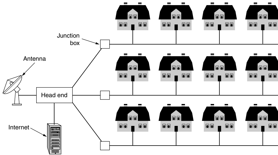
Figure 9. A metropolitan area network based on cable TV.
