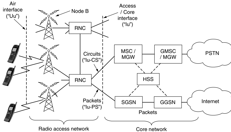
Figure 31. Architecture of the UMTS 3G mobile phone network.
