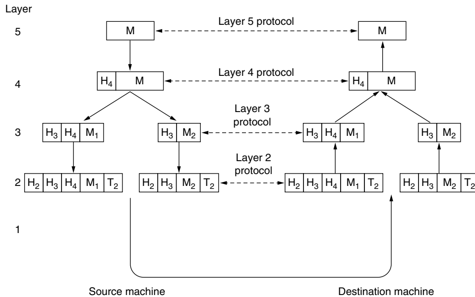
Figure 15. Example information flow supporting virtual communication in layer 5.
