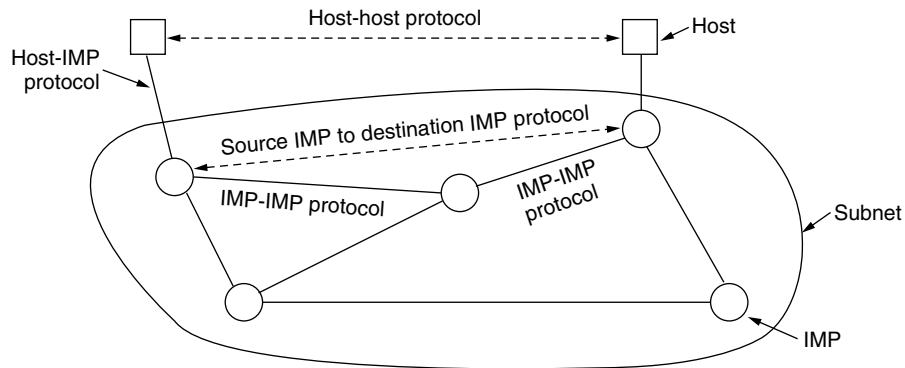
Figure 26. The original ARPANET design.
