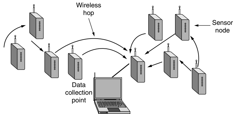
Figure 37. Multihop topology of a sensor network.
