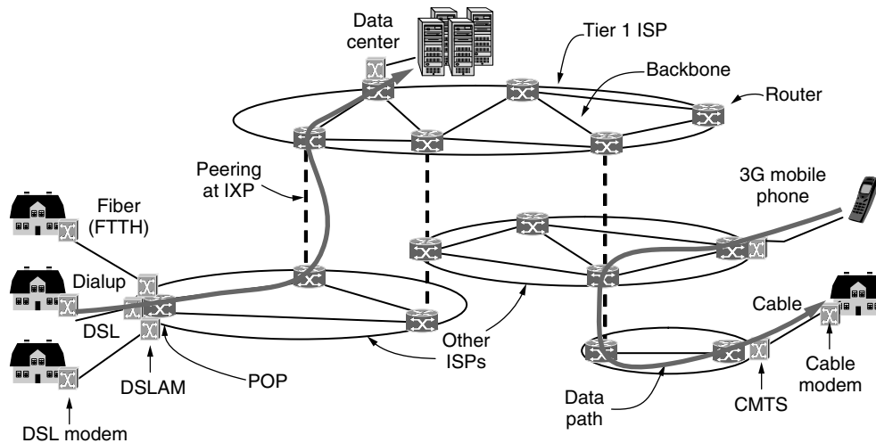
Figure 29. Overview of the Internet architecture.
