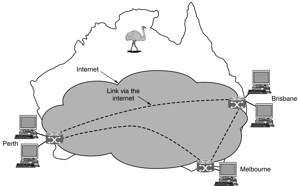
Figure 11. WAN using a virtual private network.
