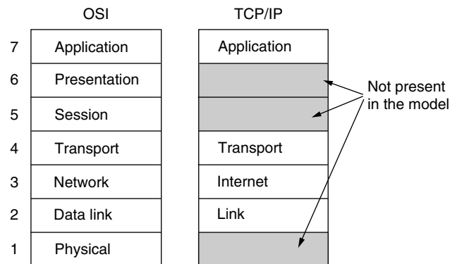
Figure 21. The TCP/IP reference model.
