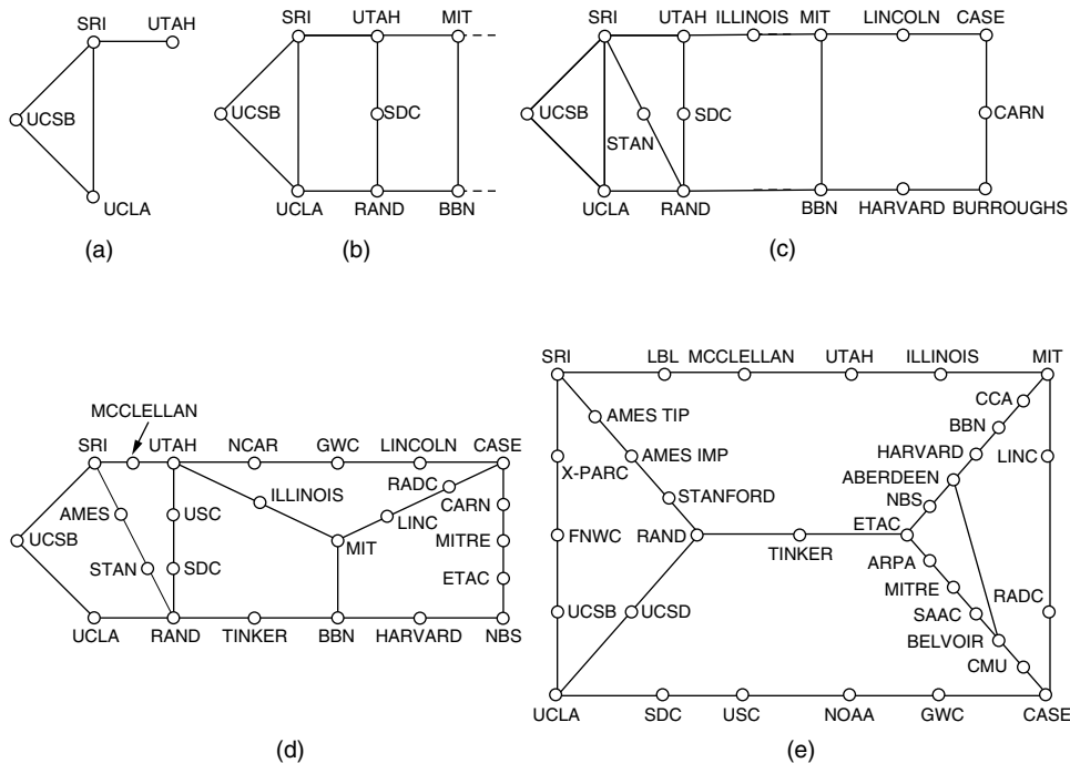
Figure 27. Growth of the ARPANET. (a) December 1969. (b) July 1970. (c) March 1971. (d) April 1972. (e) September 1972.
